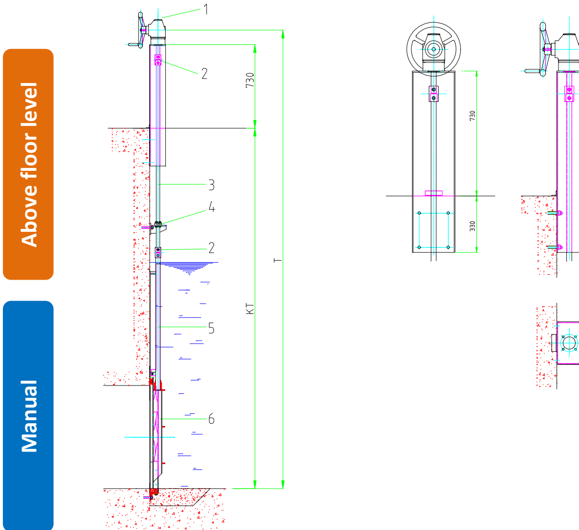
Figure with Penstock C20-Series
