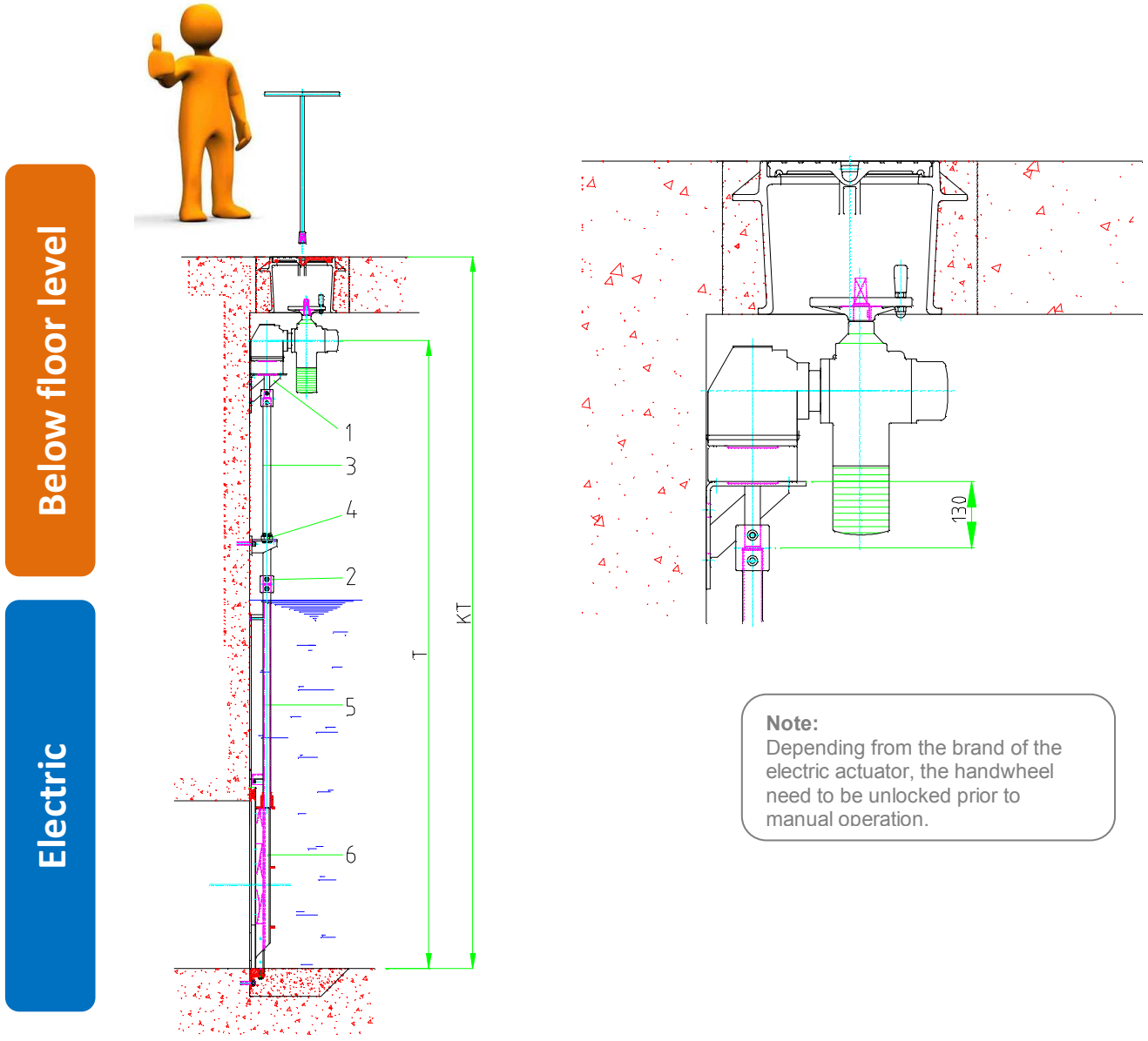
Figure with Penstock C20-Series
