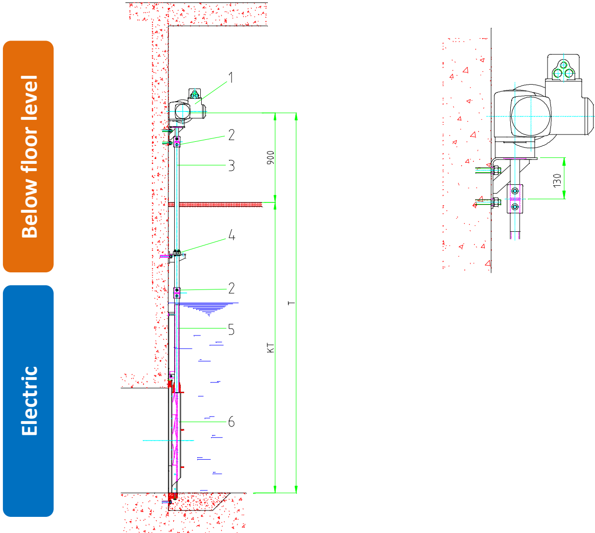
Figure with Penstock C20-Series
