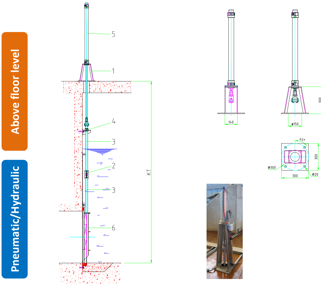
Image with pneumatic cylinder
