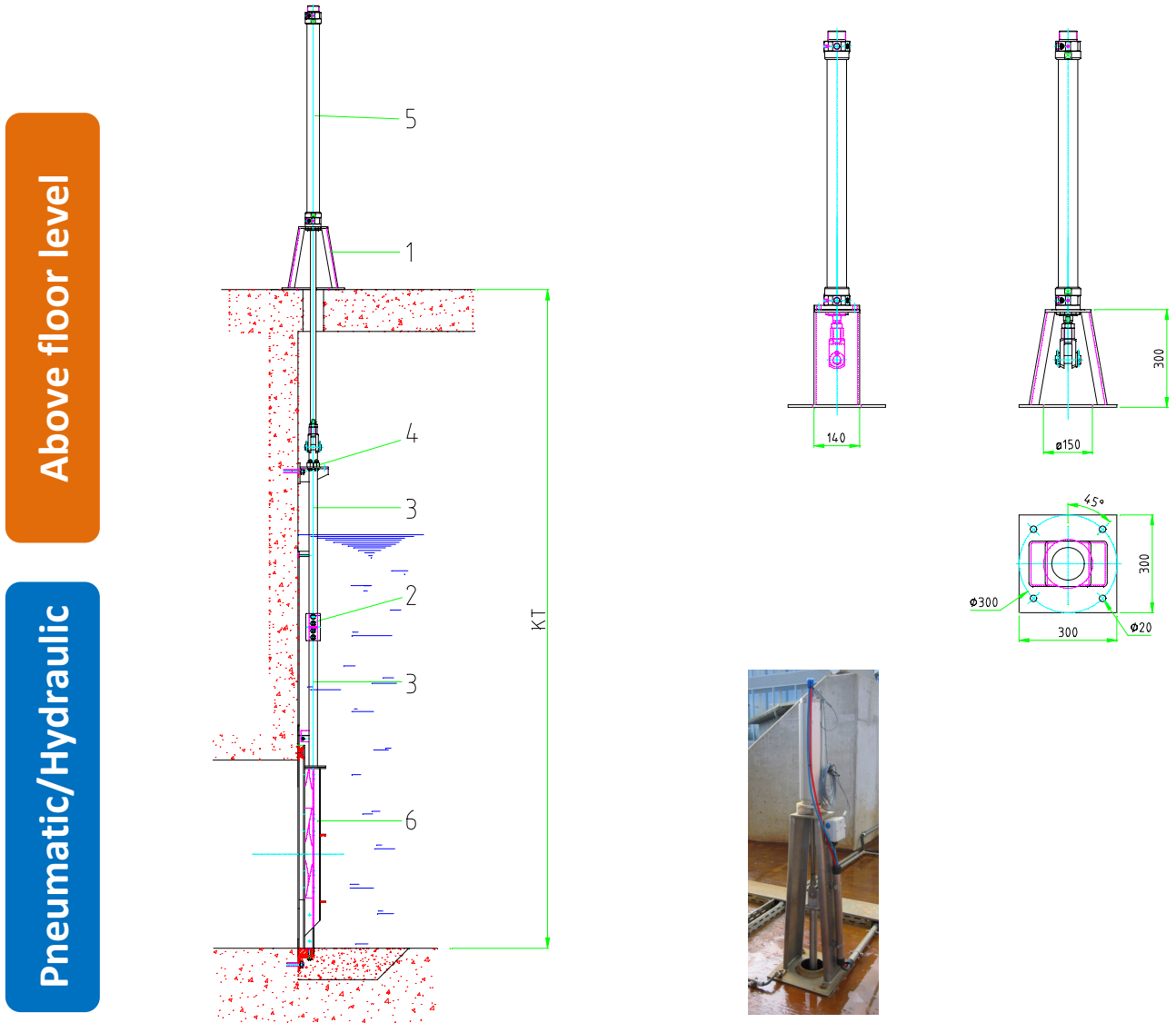
Image with pneumatic cylinder
