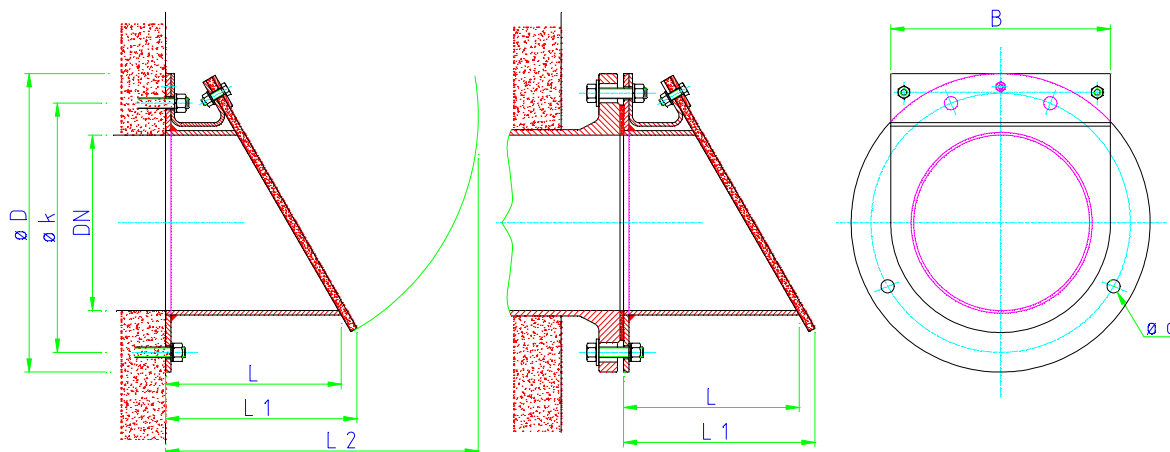
Wall fixing
