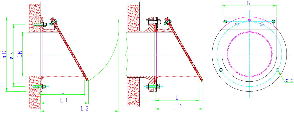
Wall fixing
